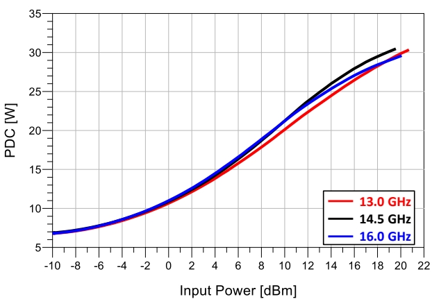
Peak Power Consumption Vs. Input Power
