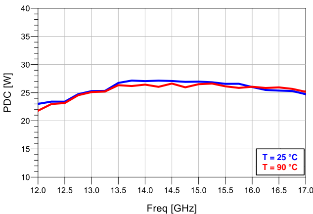
Dissipated Power Vs. Temperature
