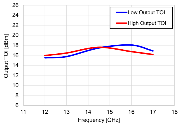
Output TOI @ -33 dBm / Tone
