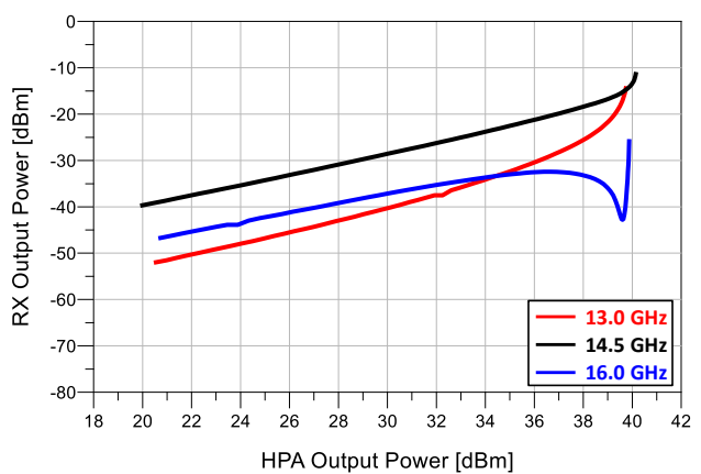
Power Leakage at RX output port Vs. TX Output Power
