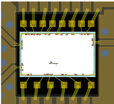
Bonding Diagram
