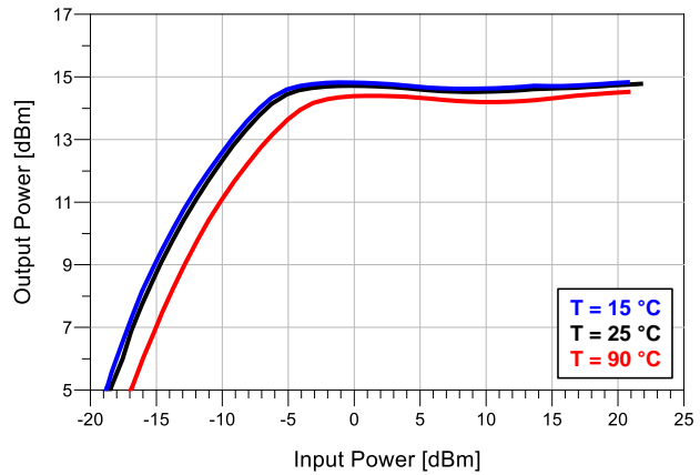
Output Power Vs. Input Power @ 13.0 GHz
