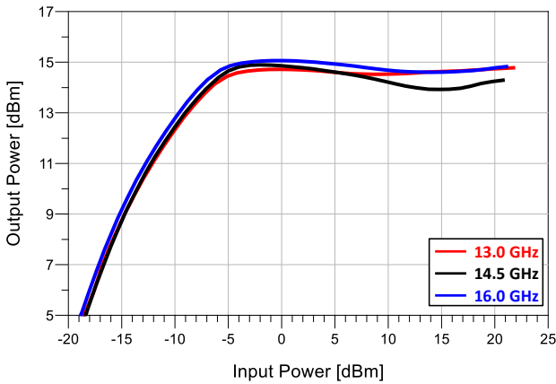
Output Power Vs. Input Power @ 25 °C
