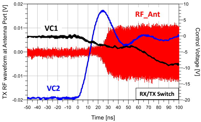
Rx to Tx switching time – RF signal @ Antenna
