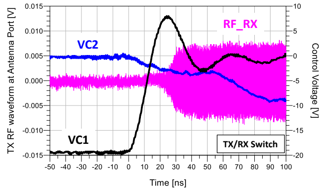
Tx to Rx switching time – RF signal @ RX port
