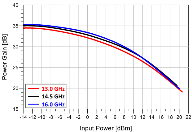
Power Gain Vs. Input Power
