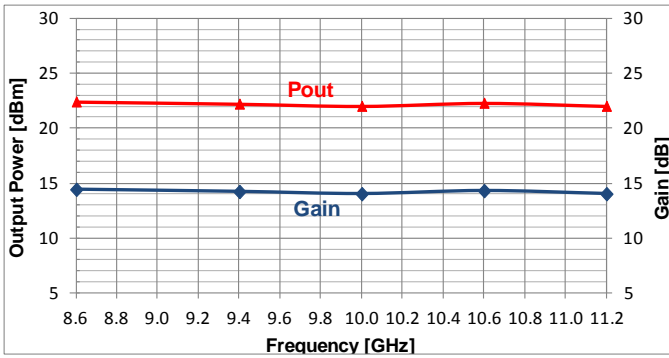
Pout and Gain Vs. Frequency @ P1dB ( P_{in} = 8\text{dBm} )
